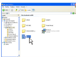
Windows XP
