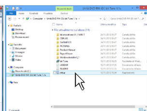
Windows 8
