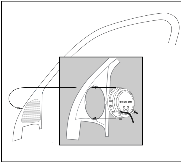
Mid-range speaker HDO-420C BMW
