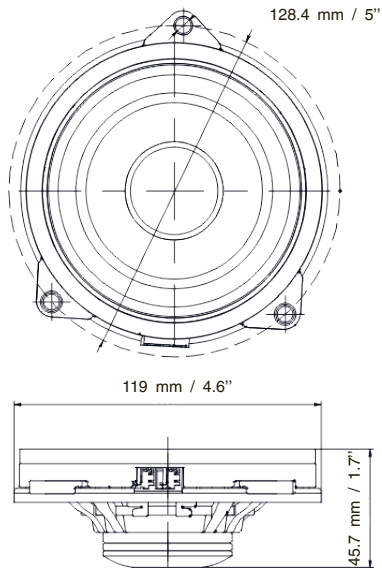
Mid-range speaker HDO-420C BMW
