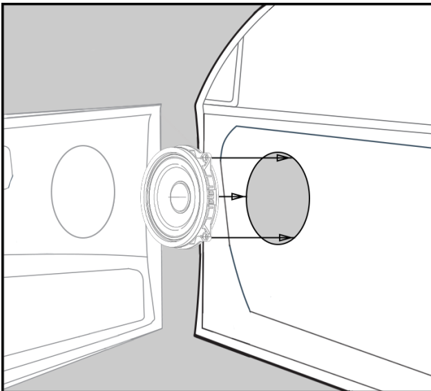
Mid-range speaker HDO-420C BMW
