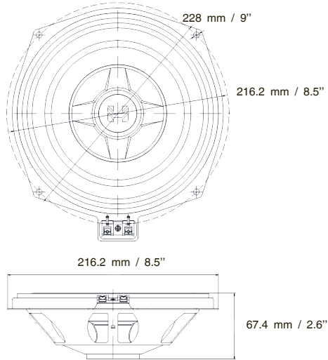
Mid-range speaker HDO-420C BMW
